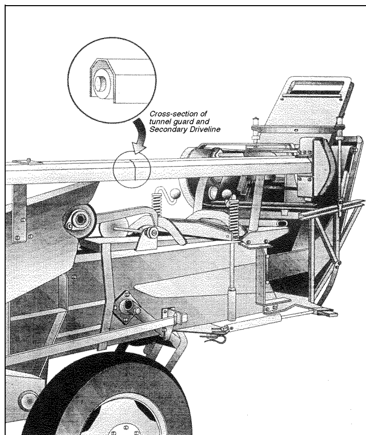
Hay baler equipped with U-shaped tunnel guard.
